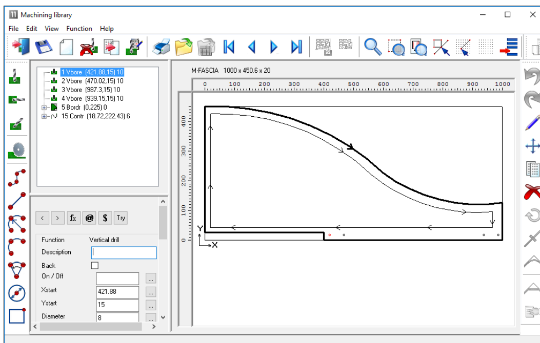
Shaped parts
